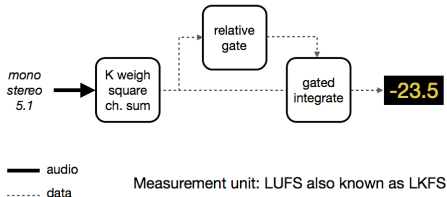
Figure 1. ITU-R BS.1770 (Program) Loudness including adaptive level-gate.
