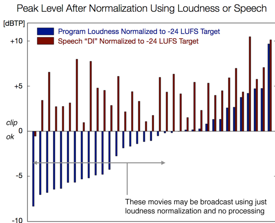
Figure 3. Max True-peak level in movies after normalization by Loudness (left bar/blue) or normalization by speech (right bar/red). Adopted from [7]
