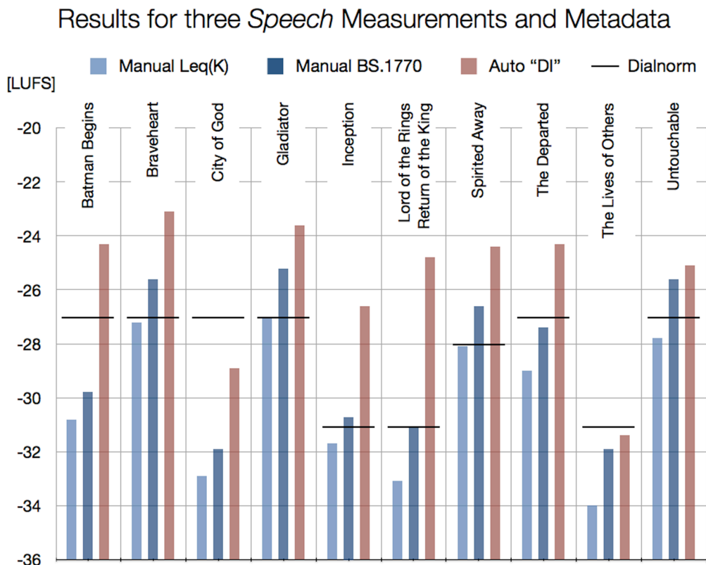
Figure 6. Measuring speech level in movies manually or automatically; and Dialnorm value on DVD.
