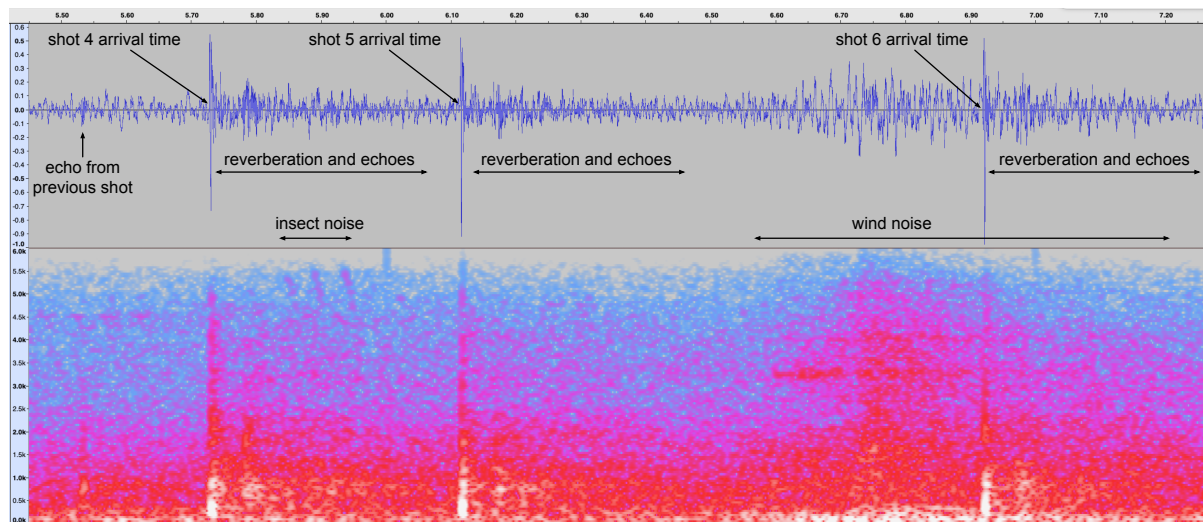
Fig. 8: Closeup waveform/spectrogram view of shots 4, 5, and 6 from sensor 1059 of #312-780375 showing the broad bandwidth of gunshot signals compared with other ambient noises. Screenshot from Audacity [24].
