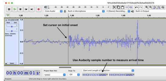
Fig. 5: Using Audacity to determine arrival time of the muzzle blast by selecting a region that starts with the first discernible increase in signal above background.
