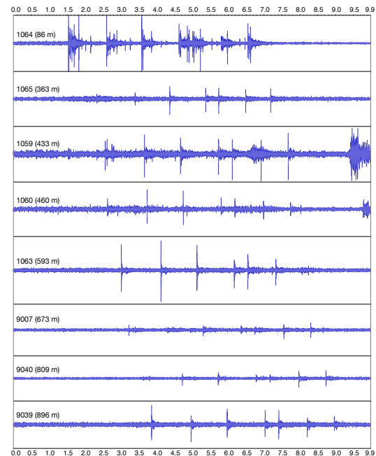
Fig. 7: Seven-shot moving shooter example (#312-780375) with waveforms sorted by distance. Audio is clock-aligned, showing the relative arrival time of the shots on each sensor.
