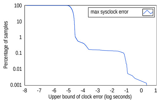
Fig. 3: Cumulative distribution function of maximum sysclock error \lambda from a survey of Scepter 2 sensors. Plotted on a log-log plot following Mills [6]. Two populations are visible, devices using KPPS refclocks ( \lambda between 10^{-5} and 10^{-4} sec) and devices using NTP refclocks ( \lambda between 10^{-3} and 10^{-1} sec); NTP refclocks are inadequate for acoustic multilateration. A small number of observations (34 out of 79119) made on devices using KPPS refclocks exhibited anomalously poor time synchronization, suggesting that timing error should be continuously monitored and recorded in audio metadata.
