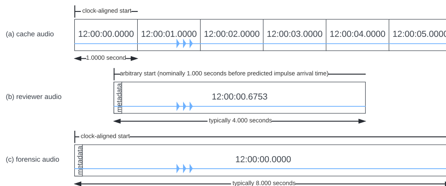
Fig. 2: Types of audio produced by the ShotSpotter system. Cache files (a) of one-second duration are recorded by the remote sensor independently of any triggering activity. Reviewer audio files (b) are constructed such that the file starts 1.0 seconds before the computed arrival time of the gunshot; forensic audio files (c) are constructed on one-second boundaries and of duration sufficient to contain all shots on all sensors.
