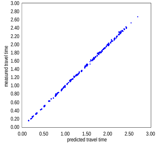
Fig. 4: Measured muzzle blast travel time ( t_i - t_o ) vs predicted travel time d_i/c .
