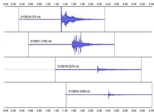
Fig. 6: Single-shot example (#783-556267) with waveforms sorted by distance. Audio is aligned to one second before the onset arrival time on each sensor.
